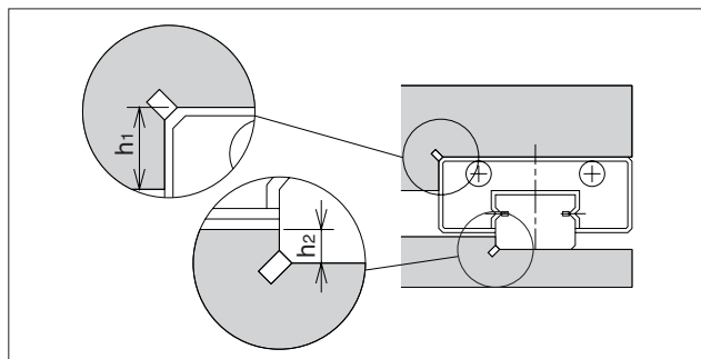
Figure A-47 Shoulder Shape-1
