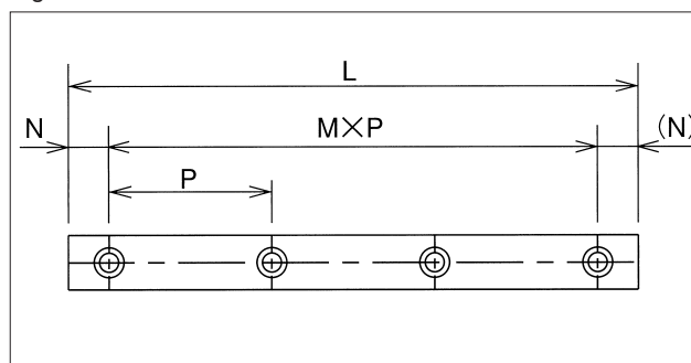
Figure A-46 Rail
