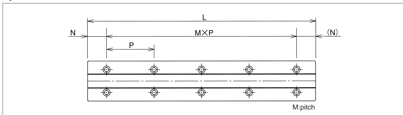
Figure A-69 Rail
