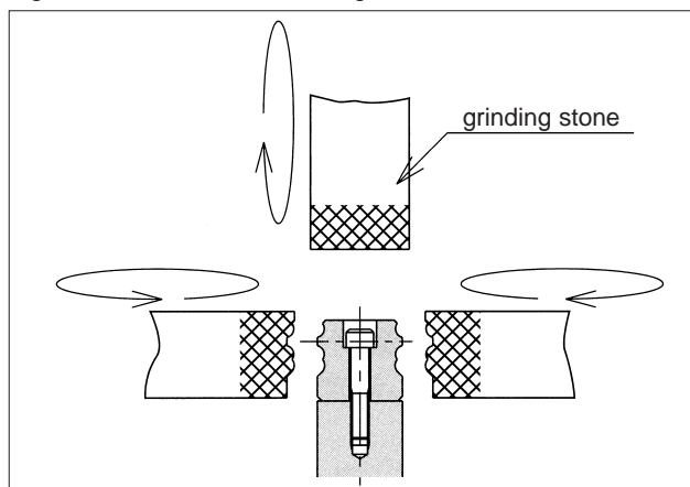
Figure A-22 Guide Rail Grinding Method
