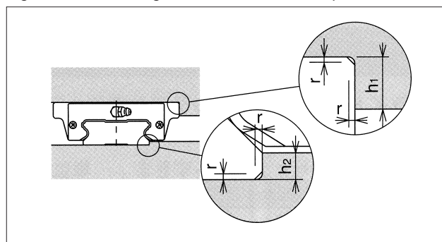
Figure A-70 Mounting Reference Surface Shapes
